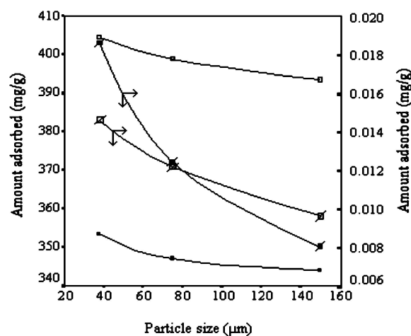
Figure 2. The effect of particle size on the removal of lignin compound and phenolic compound by fly ash and sepiolite (time: 24 h, temperature: 293 K, \text{pH} \approx 7.5 and solid/liquid: 1/50 g/mL) (■ Fly ash-phenolic compound, □ Sepiolite-phenolic compound, ▲ Fly ash-lignin compound, △ Sepiolite-lignin compound).
